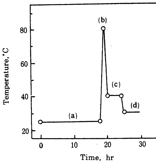
Fig.2 Temperature changes in the processes of maceration, liquefaction, saccharification and fermentation of mashed sweet potato tubers
