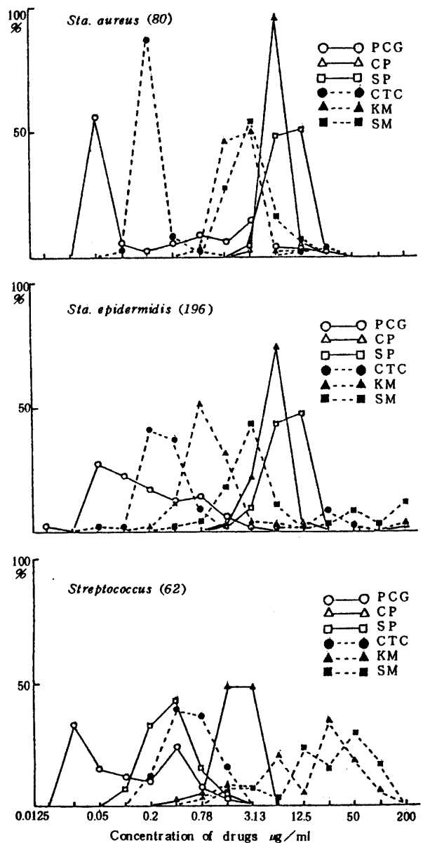
Fig. 1. Distribution curves of MIC of various drugs
