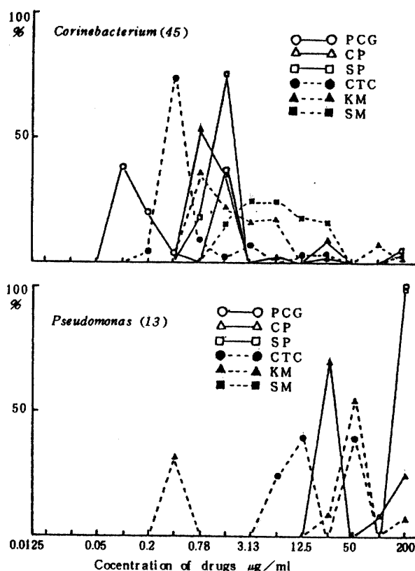
Fig. 2. Distribution curves of MIC of various drugs
