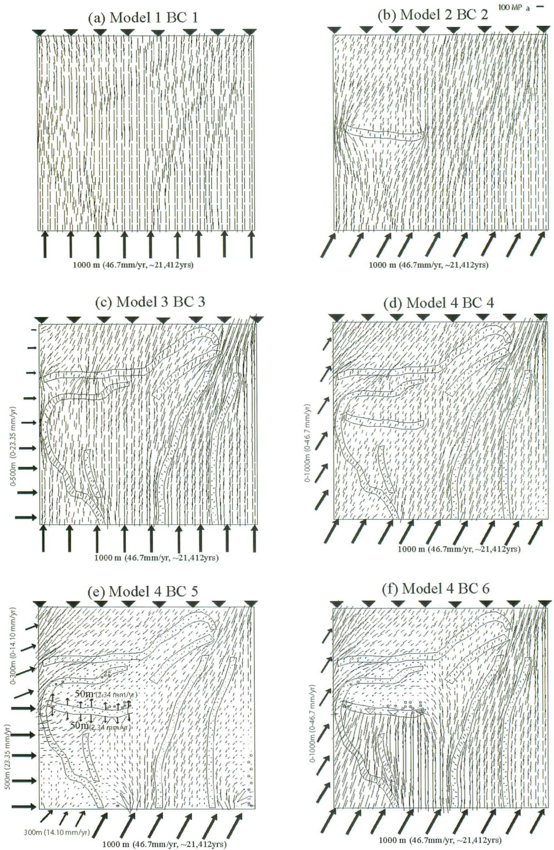
Fig. 18 Orientation of the \sigma_{Hmax} in the study area for (a) model 1 with BC 1, (b) model 2 with BC 2, (c) model 3 with BC 3, (d) model 4 with BC 4, (e) model 4 with BC 5 and (f) model 4 with BC 6 under 1000 m convergent displacement.
