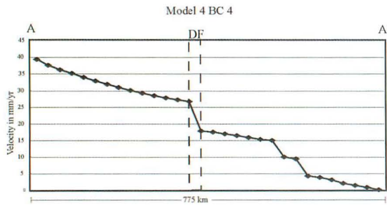
Fig. 20 N-S velocity attenuation within the model 4 under BC 4 along 91°E.
