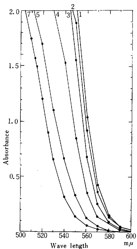
Visible absorption spectra of the solutions, between 500 and 600 millimicrons.
