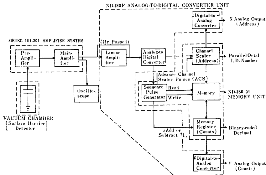
Fig. 4. Functional block diagram for alpha-particle measurement system
