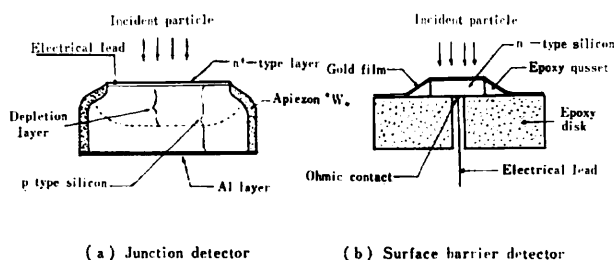
Fig. 3. Schematic diagram of semiconductor detector
