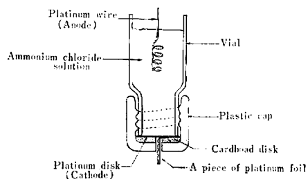
Fig. 2. Electroplating cell
