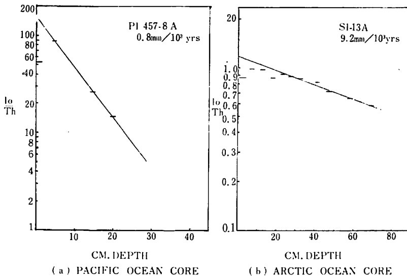
Fig. 9. The ionium/thorium ( \text{Th}^{230}/\text{Th}^{232} ) ratios as a function of depth
