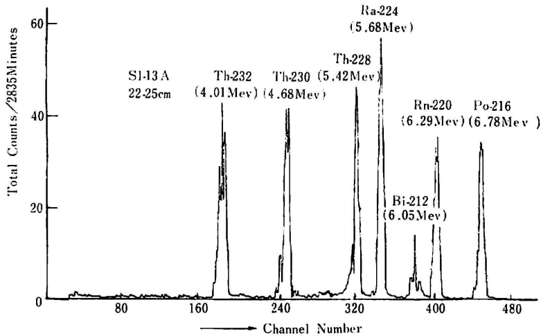
Fig. 5. The alpha-spectrum of thorium isotopes isolated from arctic ocean core
