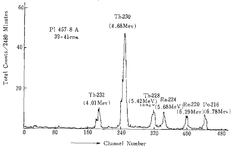
Fig. 8. The alpha-spectrum of thorium isolated from pacific ocean core
