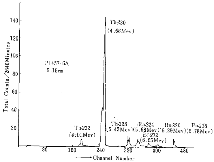
Fig. 7. The alpha-spectrum of thorium isotopes isolated from pacific ocean core
