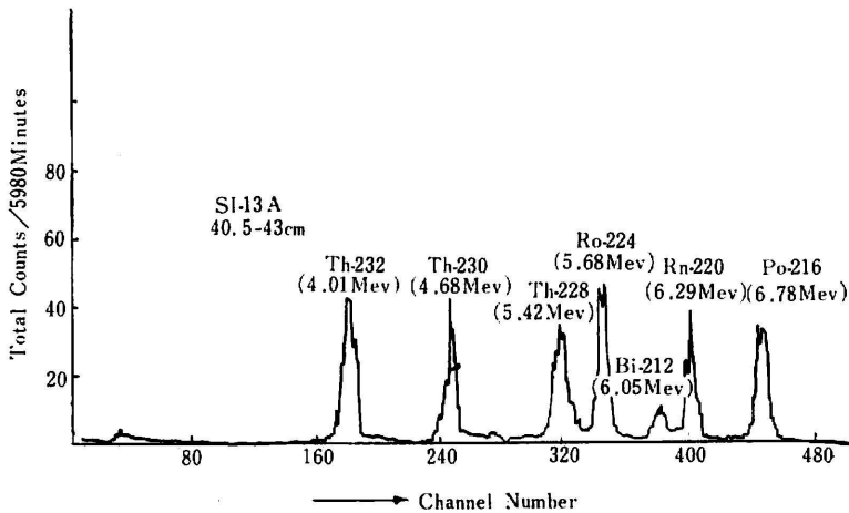
Fig. 6. The alpha-spectrum of thorium isotopes isolated from arctic ocean core
