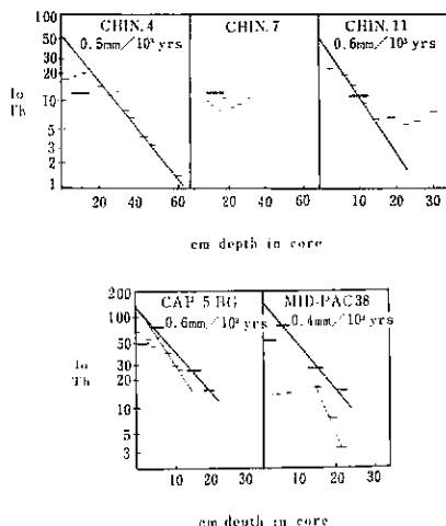
Fig. 10. Profiles of the ionium/thorium ( \text{Th}^{230}/\text{Th}^{232} ) ratio in sediment samples from the pacific ocean*
