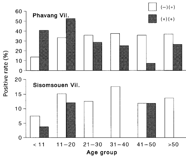
FIGURE 1. Relation of the results from microscopical examination and polymerase chain reaction (PCR) assay for malaria infection by age group. (-)(+) indicates that the specimen was negative by microscopic examination and positive by PCR assay. (+)(+) indicates the specimen was positive by both methods.
