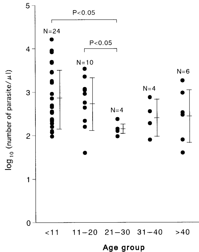
FIGURE 2. Comparison of number of malaria parasites among positive smears by age group in Phavang Village.
